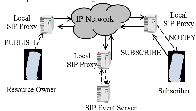
Fig. 2. SIP Event Architecture
